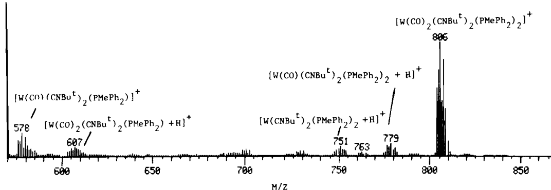
Fig. 1. FAB-MS (high mass region only) of W(CO)_2(CNBu^t)_2(PMePh_2)_2 from a 1:1 dithiothreitol/dithioerythritol matrix. The cluster of peaks at m/z 806 is probably due to a combination of [W(CO)_2(CNBu^t)_2(PMePh_2)_2]^+ ( m/z 806) and [W(CO)_2(CNBu^t)_2(PMePh_2)_2 + H]^+ ( m/z 807) ions.
